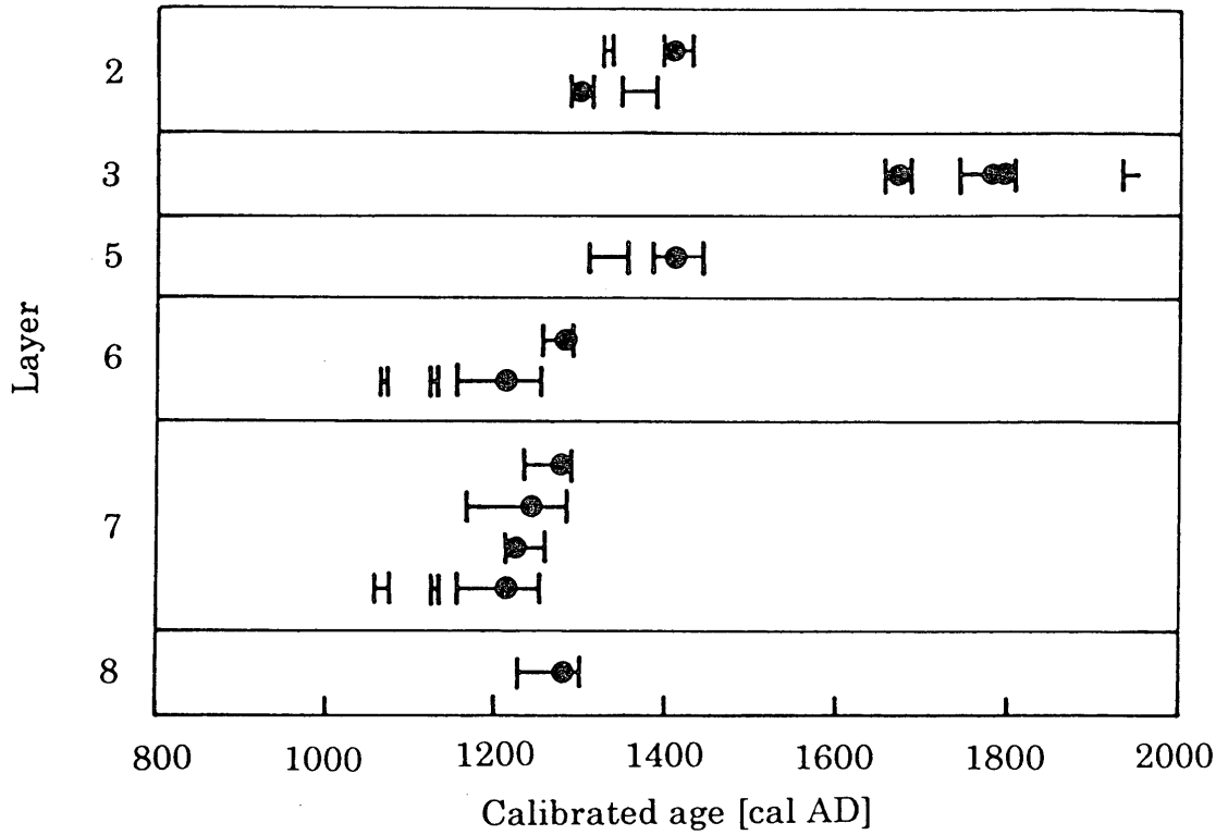
Fig. 1. Calibrated dates from 14 C ages measured for charcoal samples excavated from Viroronga(V.R.)-A site in 1993.
