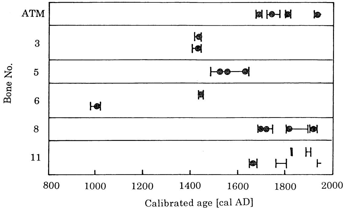
Fig. 2. Calibrated dates from 14 C ages measured for charcoal samples excavated from Viroronga(V.R.)-C site in 1993-1994.
